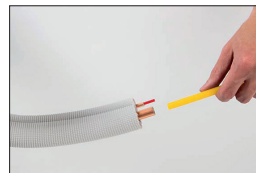
STEP 3 Retract the flexible bender.
